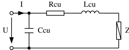
Figure 9: Complete equivalent electrical circuit
